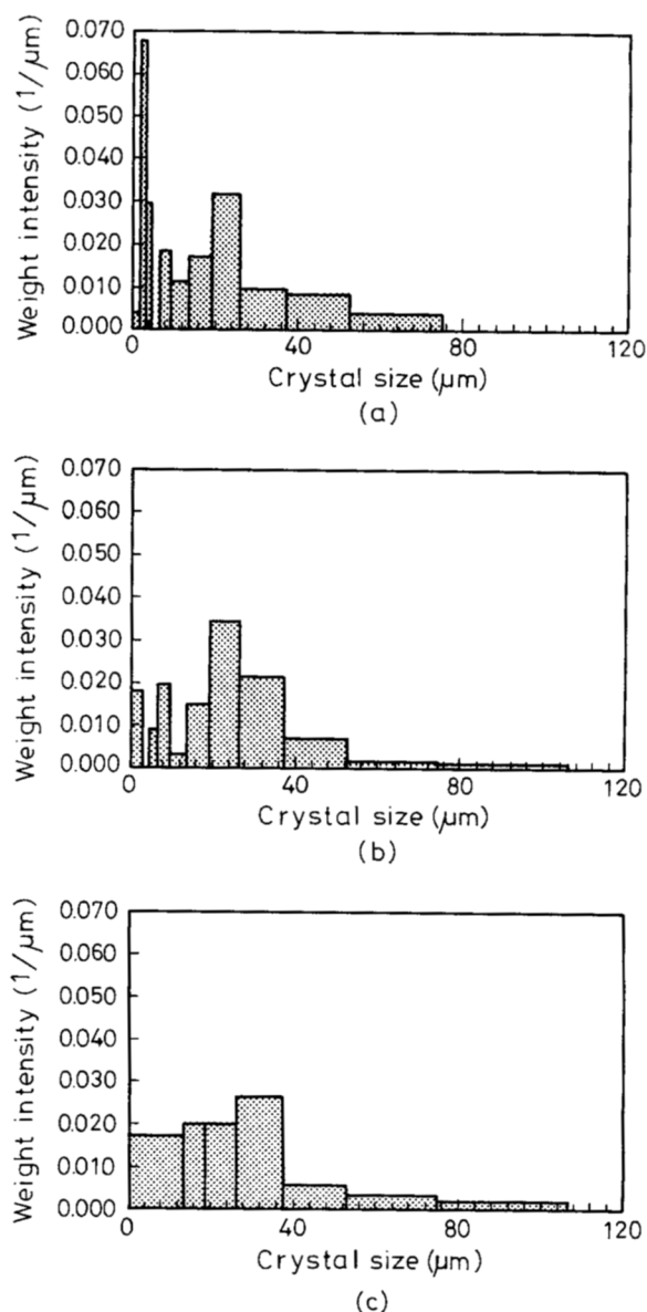
Figure 5. Crystal-size distributions in the pH-stat semi-batch study at the same operating conditions except the amount of seed.
