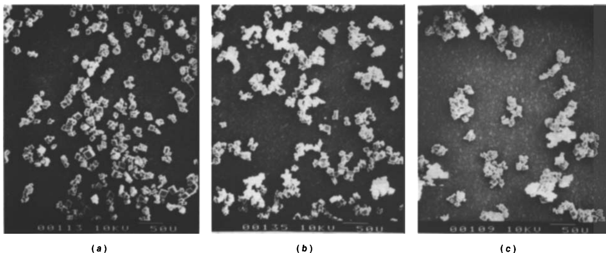
Figure 6. SEM photographs of calcite obtained from contact mechanism in the pH-stat semibatch study at various amount of seeding.
